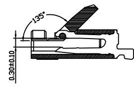
SECTION B-B SCALE 1:1 When Cover Is Opene
