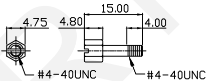
Screw Specification
