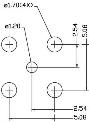
PCB MOUNTING HOLES
