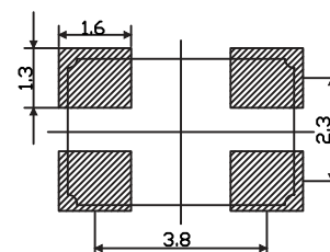
Example of a Terminal Land Pattern
